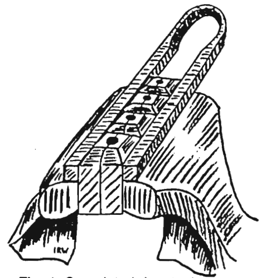
Fig. 4 Completed rivet tool shown in vise
